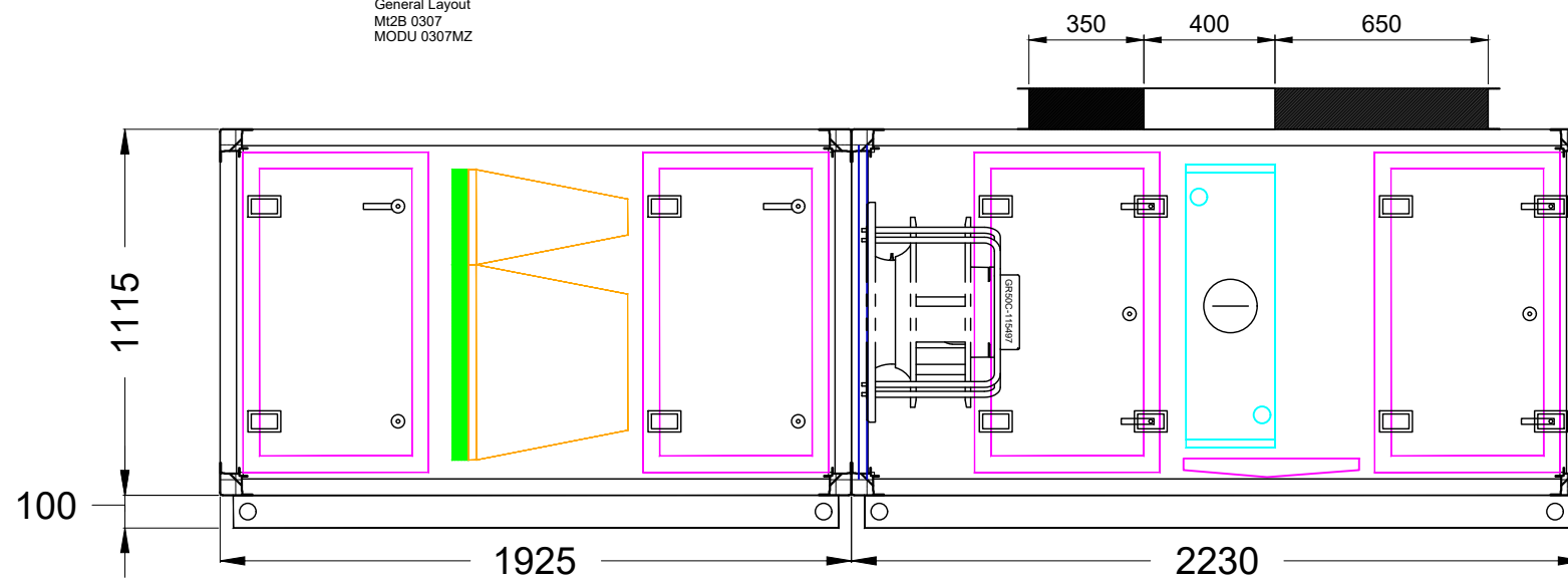
Right View
