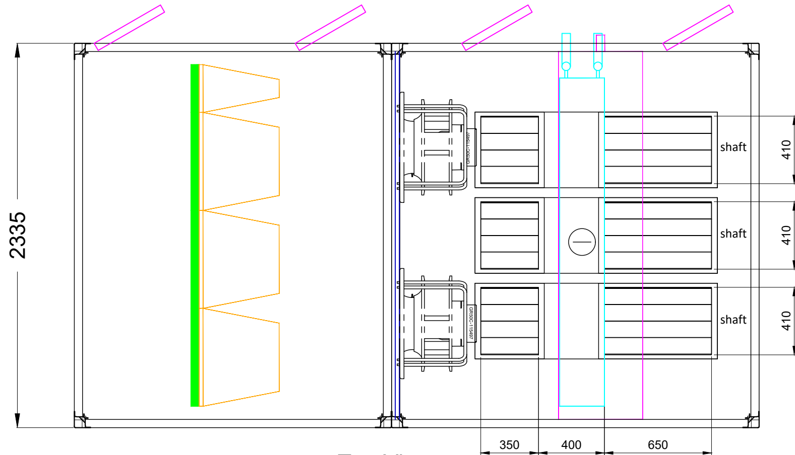
Top View
